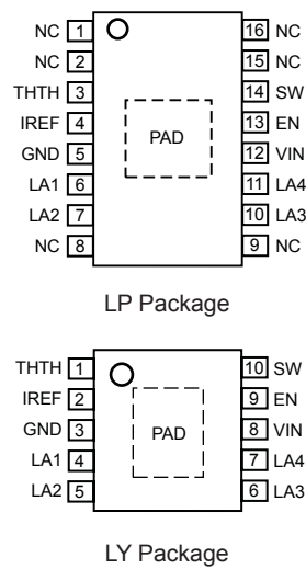
Pin-out Diagrams
