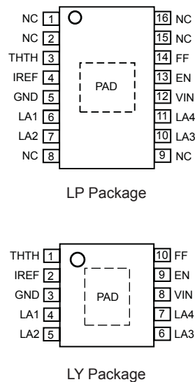
Pin-out Diagrams
