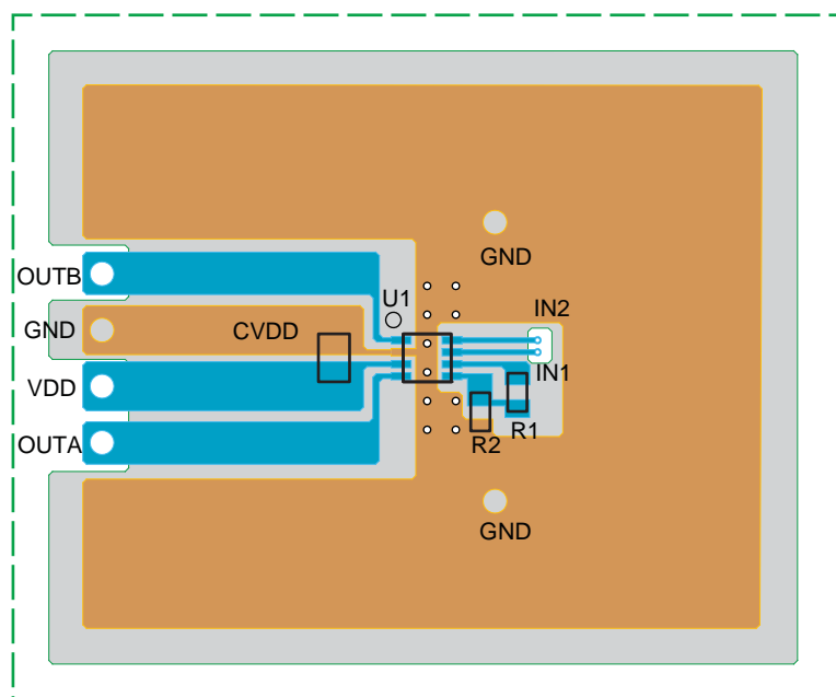
A3903 Evaluation Board
