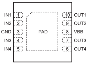
Terminal Diagram
