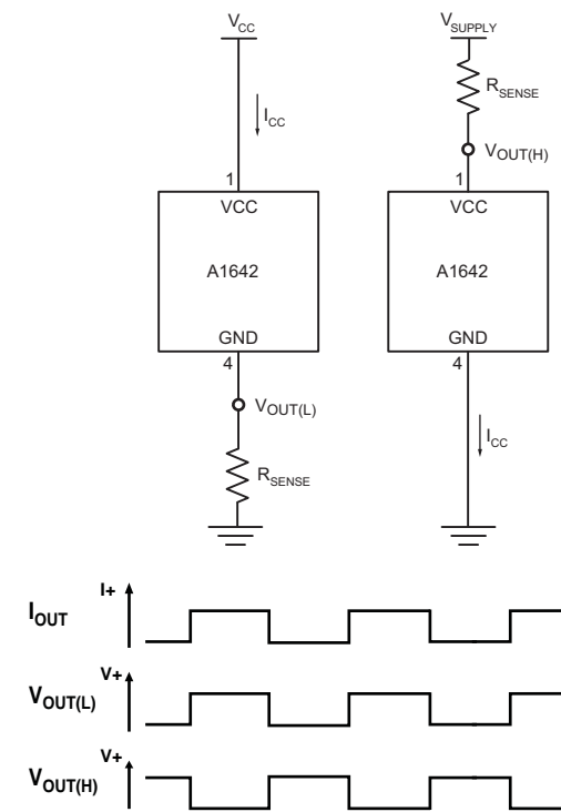
Figure 4: Voltage profiles for high side and low side two-wire sensing.
