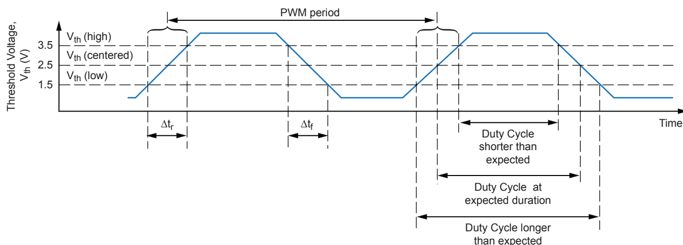
Figure 12. When the threshold voltage, V_{th} , is correctly centered between V_{th}(\text{high}) and V_{th}(\text{low}) , the current duty cycle accurately coincides with the applied magnetic field. If the threshold voltage is raised, the current duty cycle appears shorter than expected. Conversely, if the threshold voltage is lowered, the current duty cycle is longer than expected.
