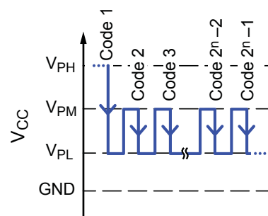
Figure 6. Try mode bit field addressing pulses.
