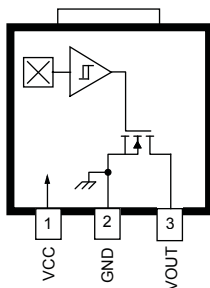
LT Package
