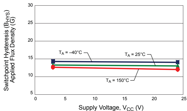
Average Hysteresis (South) versus Supply Voltage
