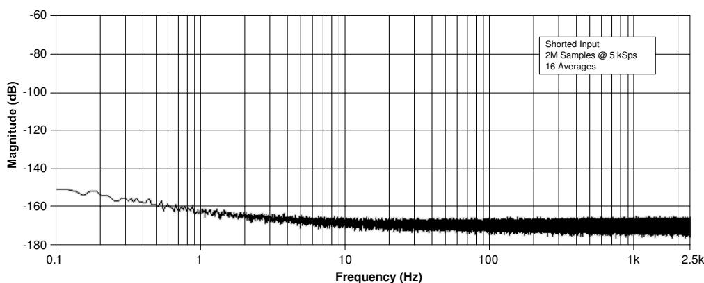
Figure 18. Spectral Plot of Noise with Shorted Input
