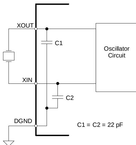
Figure 8. Oscillator Connection
