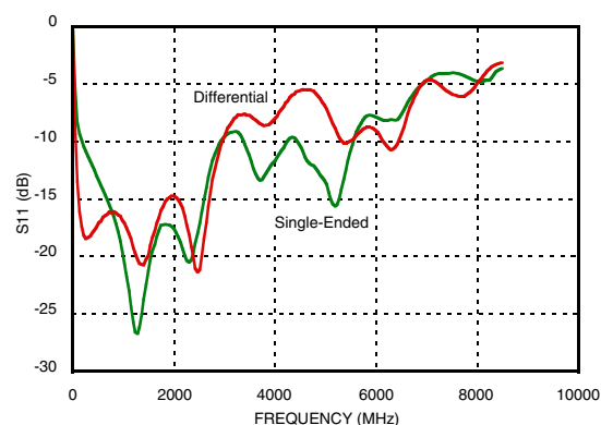
Figure 20. S-Parameters - S11 [11]
