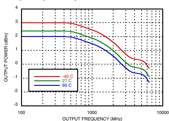
Figure 9. Fundamental Output Power vs. Frequency & Temperature [6]
