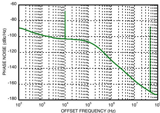
Figure 11. HMC984LP4E & HMC983LP5E PLL Performance at 7000.01 MHz [4]
