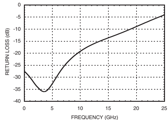
Clock Output Return Loss vs. Frequency [1][3][4]
