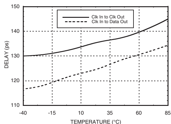
Delay vs. Temperature [1][3]
