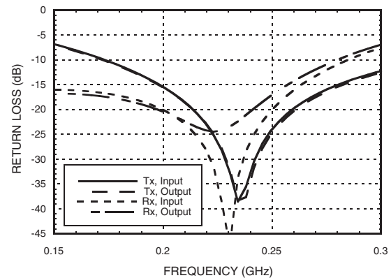
Return Loss with 220 MHz Tuning
