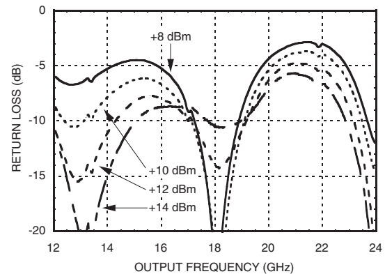
Output Return Loss with 12 GHz Input
