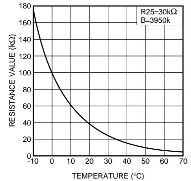
Fig. 5 Thermistor curve
