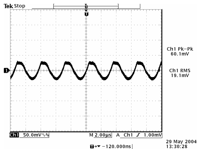
Ripple and noise at full load, V_{in}=12 V, V_o=6.0 V
