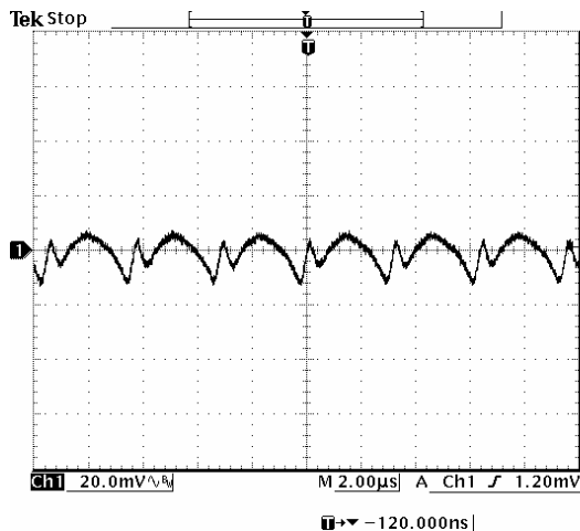
Ripple and noise at full load, V_{in}=12 V, V_o=0.75 V
