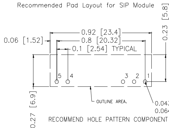
Recommended Pad Layout for SIP Module
