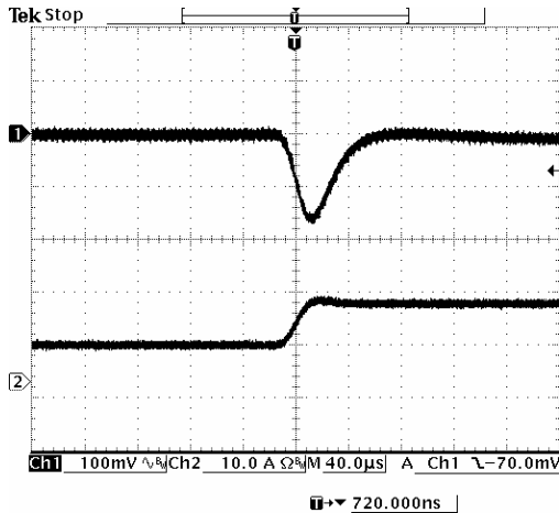
50% to 100% load Transient at Vin=5 V, Vo=1.8 V
