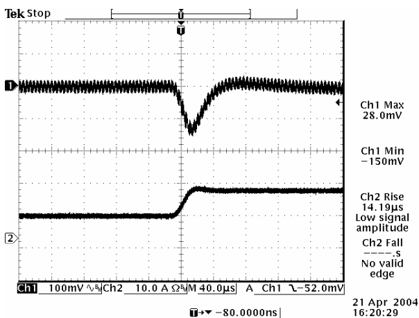
50% to 100% load Transient at Vin=12 V, Vo=2.5 V
