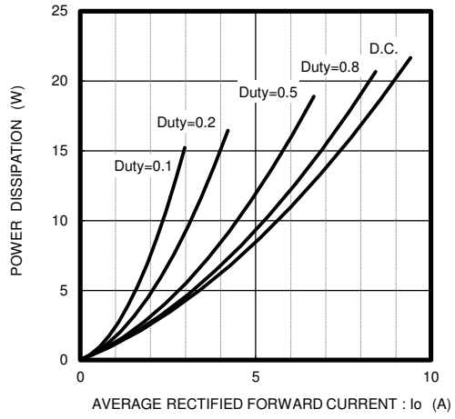
Fig.8 Io-Pf Characteristics
