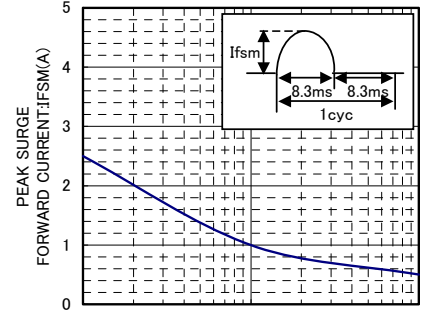
IFSM-CYCLE CHARACTERISTICS
