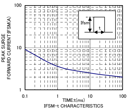
IFSM-t CHARACTERISTICS
