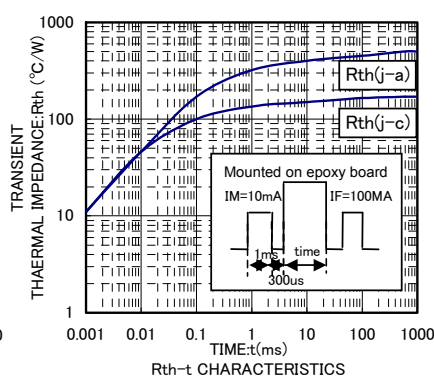
Rth-t CHARACTERISTICS
