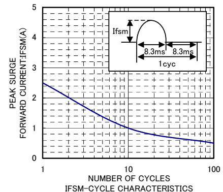
IFSM-CYCLE CHARACTERISTICS
