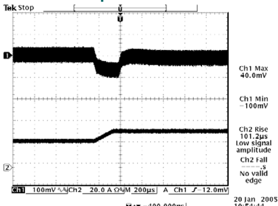
Vout=3.3 V, 50% to 75% Load Transients
