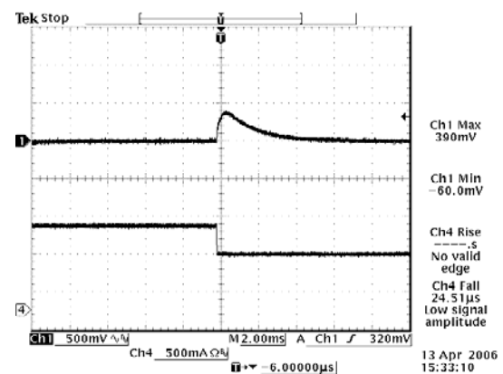
75%-50% Load Transients at V_{in}=48\text{ V} , V_o=54\text{ V}
