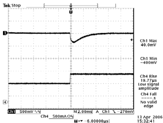
50%-75% Load Transients at V_{in}=48\text{ V} , V_o=54\text{ V}
