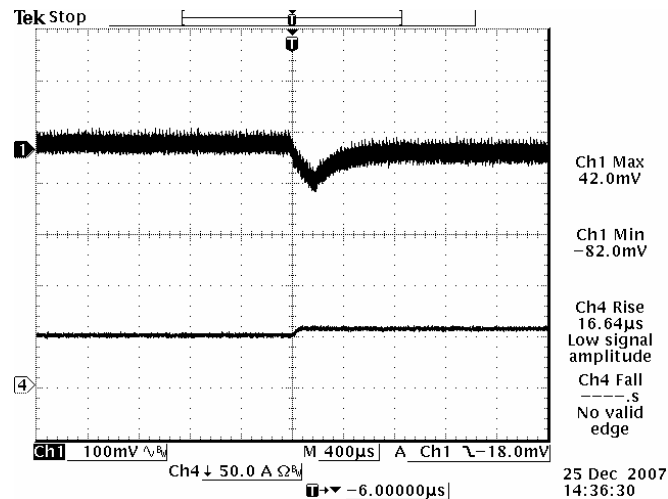
50%-75% Load Transients at V_{in}=48 V
