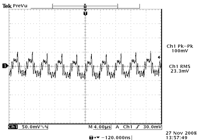
24 Vdc input, 12 Vdc/12 A output
