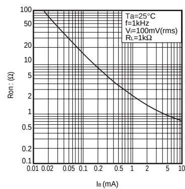
Fig.12 Output on resistance vs. base current
