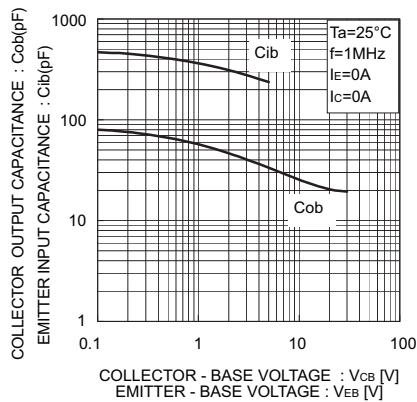
Fig.7 Emmitter Input Capacitance vs. Emmitter-Base Voltage Collector Output Capacitance vs. Collector-Base Voltage
