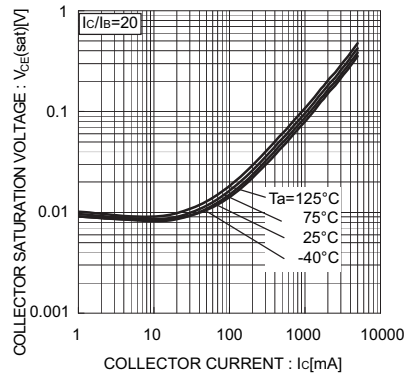
Fig.5 Collector-Emmitter Saturation Voltage vs. Collector Current ( II )
