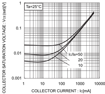
Fig.4 Collector-Emmitter Saturation Voltage vs. Collector Current ( I )
