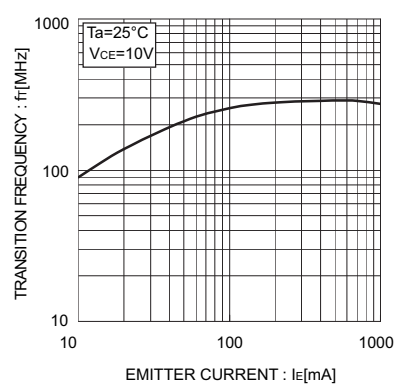
Fig.8 Gain Bandwidth Product vs. Emmitter Current
