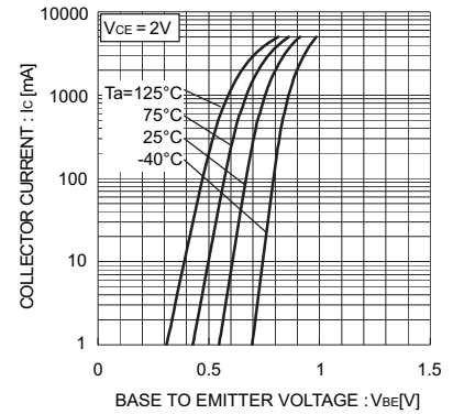
Fig.6 Ground Emmitter Propagation Characteristics
