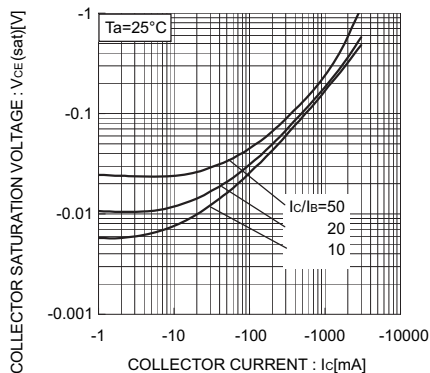
Fig.4 Collector-Emitter Saturation Voltage vs. Collector Current ( I )
