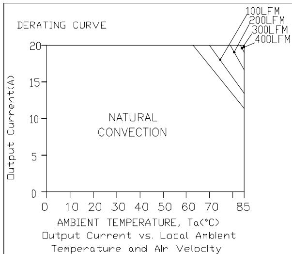
Derating curve under 48V input
