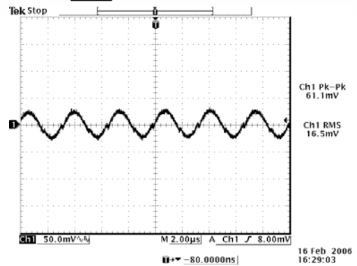
V_{in} = 48\text{ V} and I_{out} = 25\text{ A}
