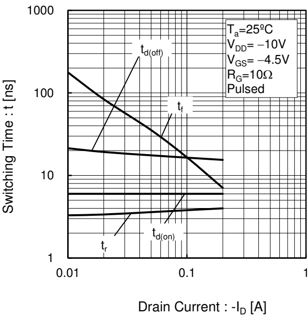
Fig.18 Switching Characteristics
