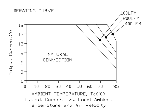
xRSB-40UV2x, Vin=48V
