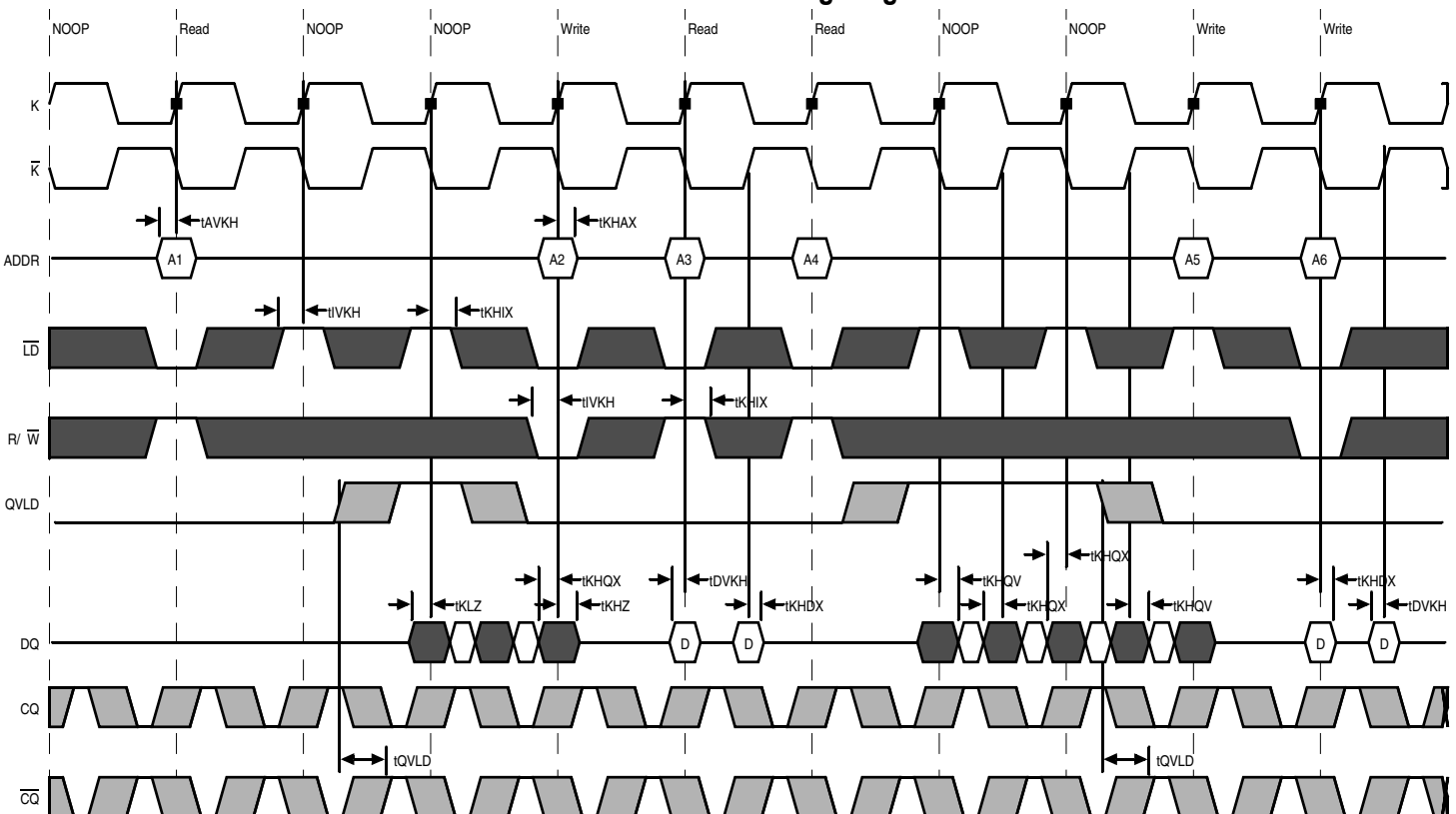
Read-Write K-Based Timing Diagram
