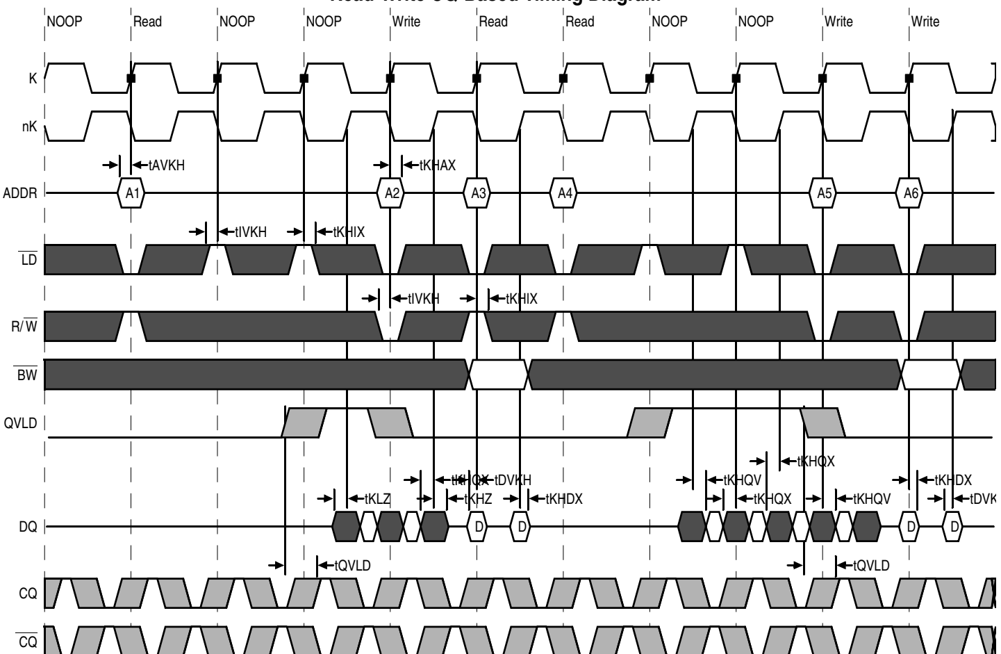
Read-Write CQ-Based Timing Diagram
