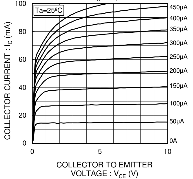
Fig.2 Grounded emitter output characteristics I_B = 500\mu\text{A}
