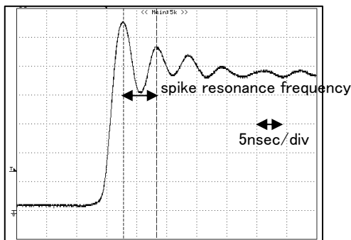
Figure .35 PWM Output waveform (measure of spike resonance frequency)
