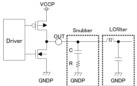
Figure .36 snubber schematic
