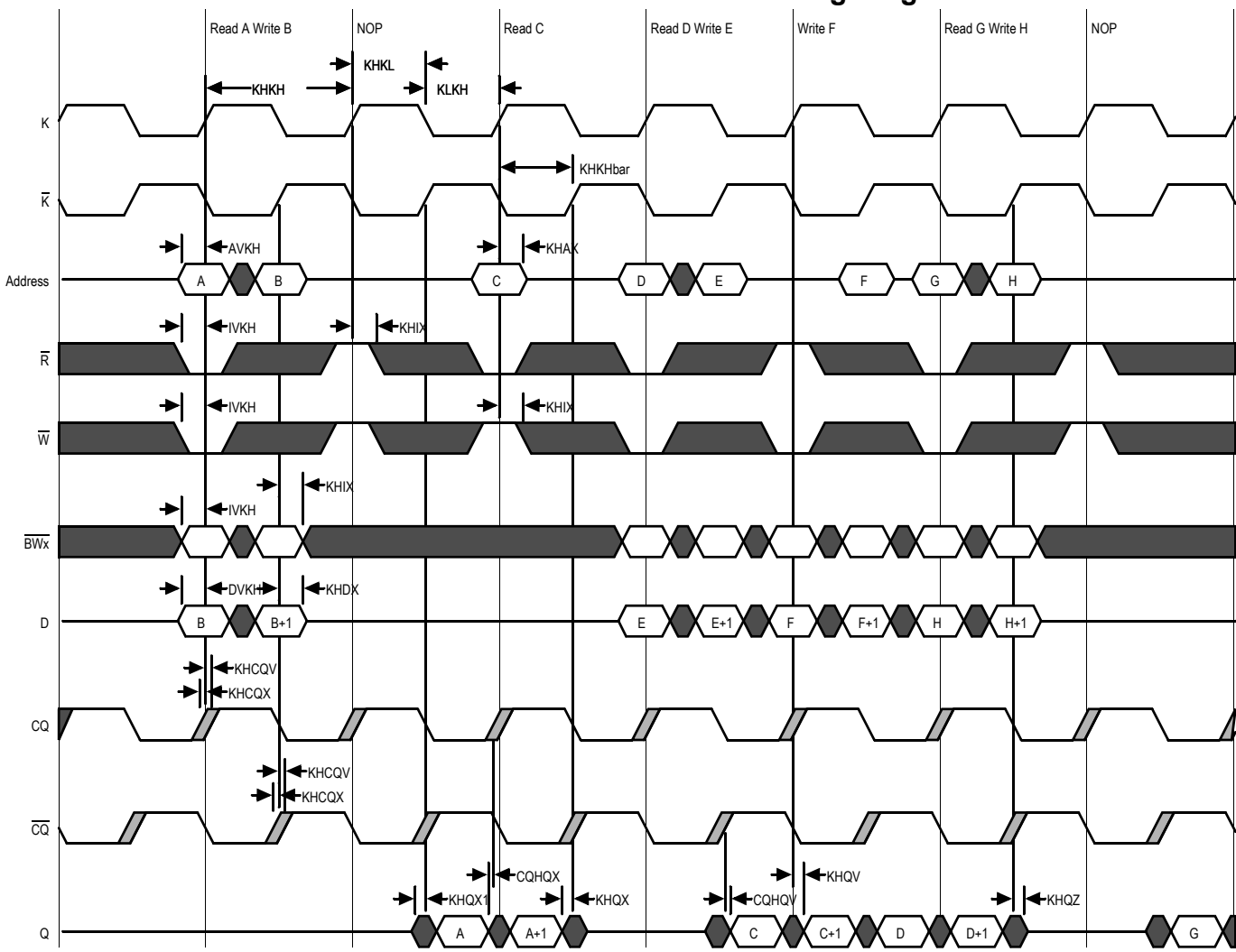
K and \overline{K} Controlled Read-Write-Read Timing Diagram
