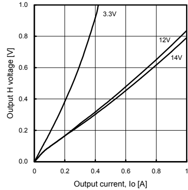
Fig.7 Output H voltage (Voltage characteristics)
