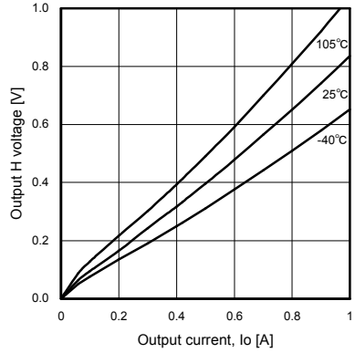
Fig.8 Output H voltage (Temperature characteristics)
