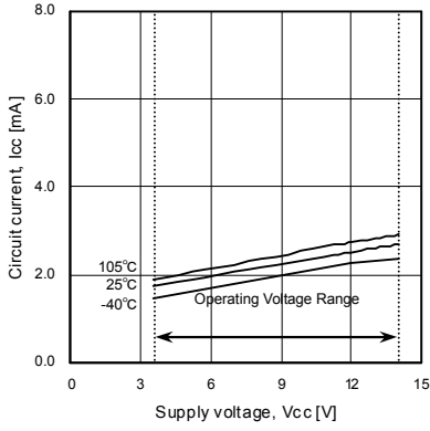
Fig.1 Circuit current 1
