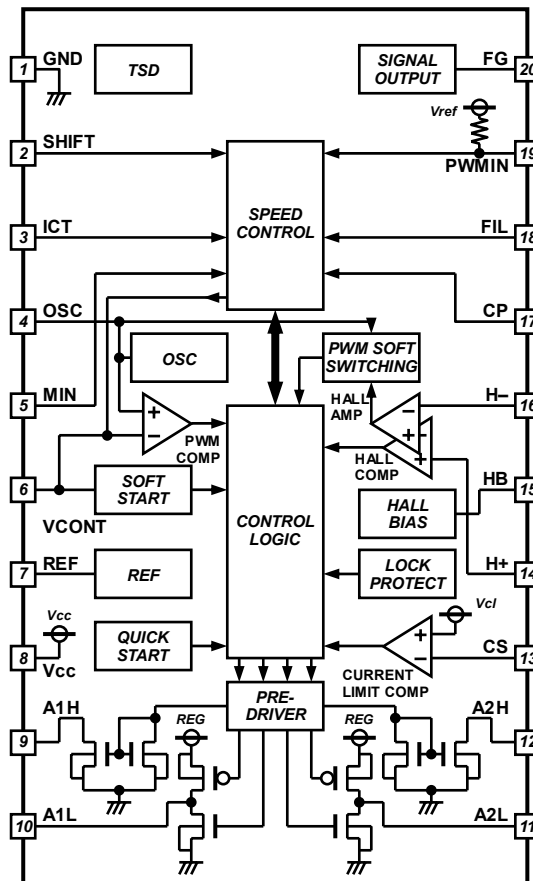
Fig.2 Block diagram
