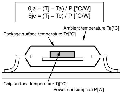
Fig.34 Thermal resistance
