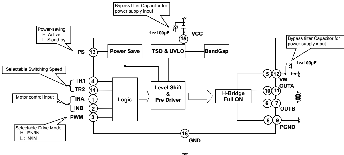
Figure 1. Block Diagram / Application Example
