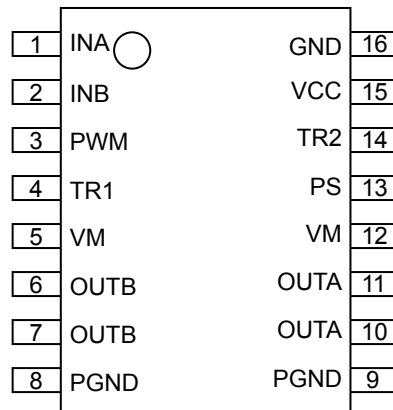
Figure 2. Pin Configuration (Top View)
