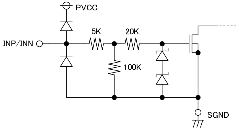
Figure10: Input circuit diagram
