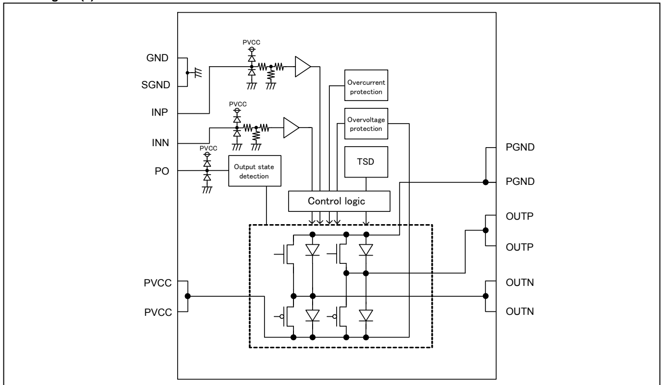
Figure3: Block Diagram
