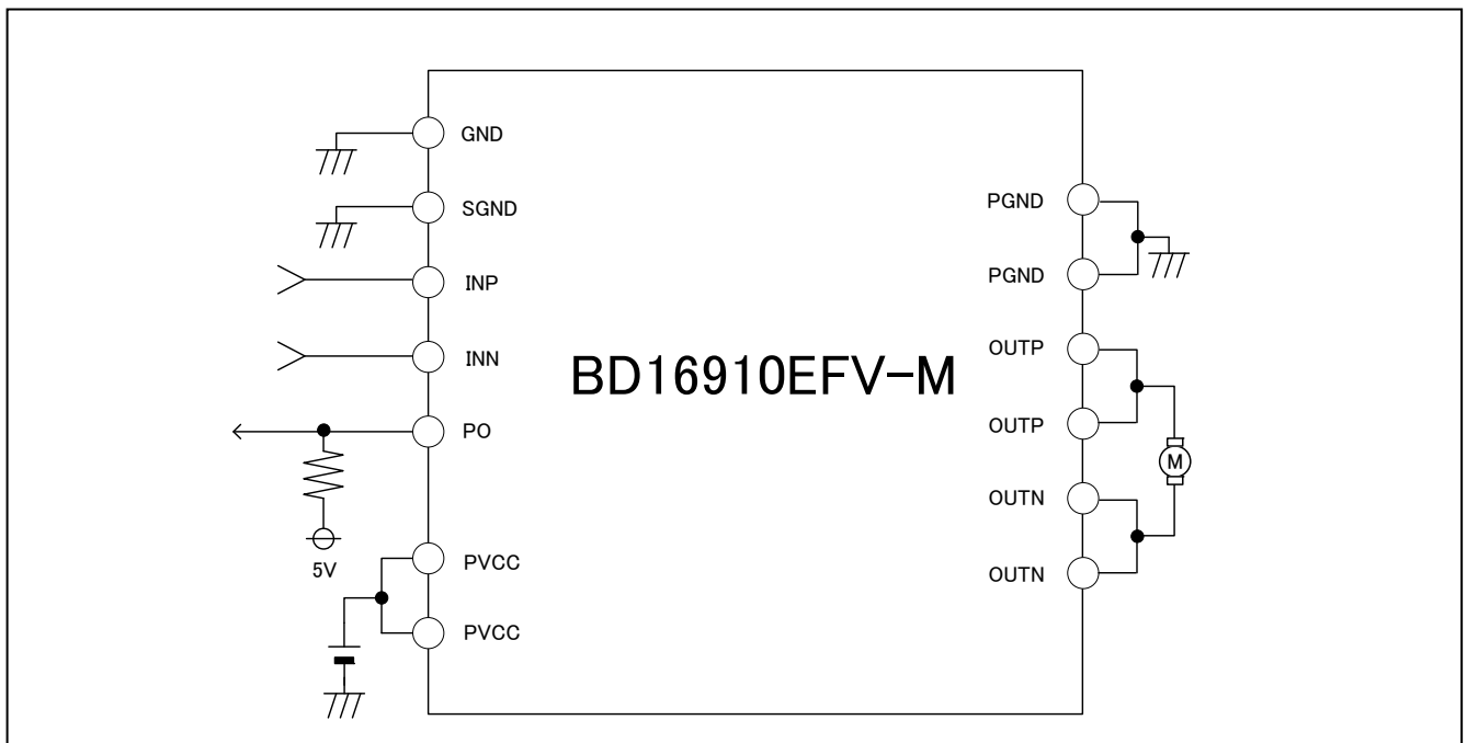
Figure1:Typical Application Circuits
