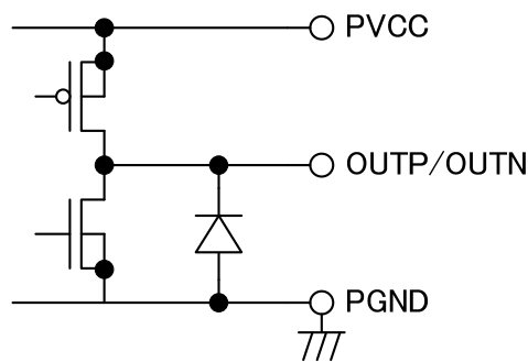
Figure12: Output circuit diagram
