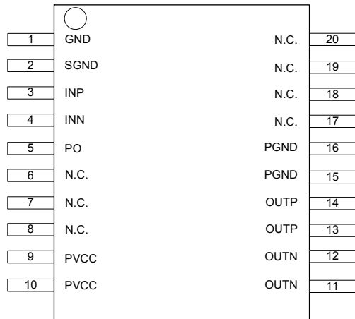
Figure2: Pin Configuration
