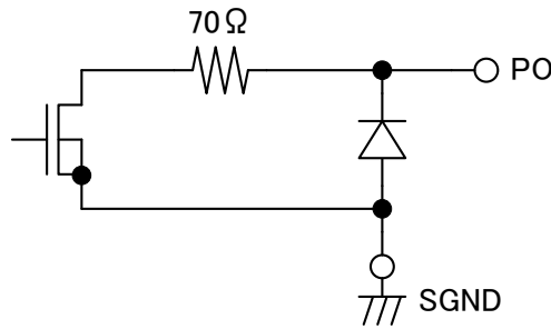
Figure11: PO circuit diagram
