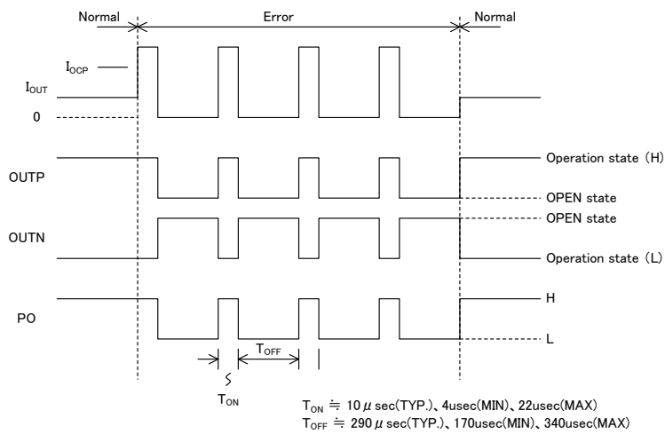
Figure4: PO timing chart (INP=H, INN=L at normal rotation)
