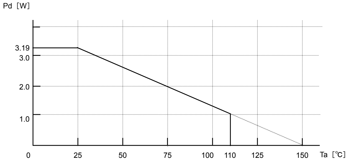
Figure8: BD16910EFV-M Power dissipation
