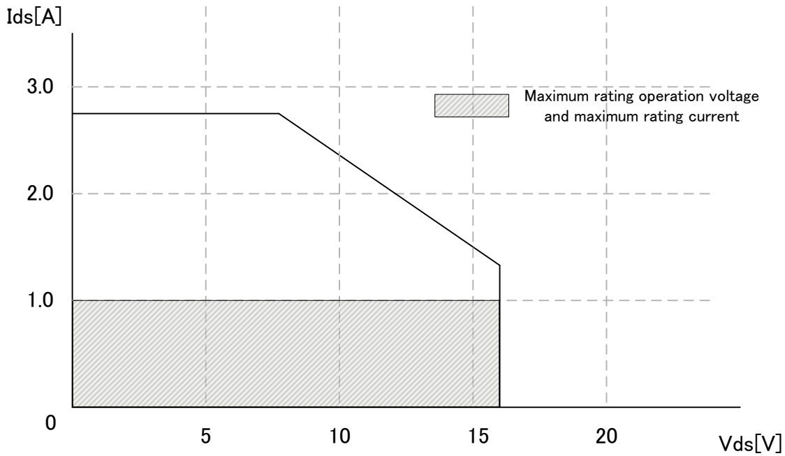
Figure9: BD16910EFV-M ASO characteristic
