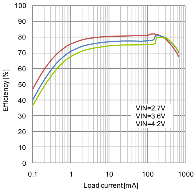
Figure 17. Efficiency vs Load current PWM/PFM Auto mode
