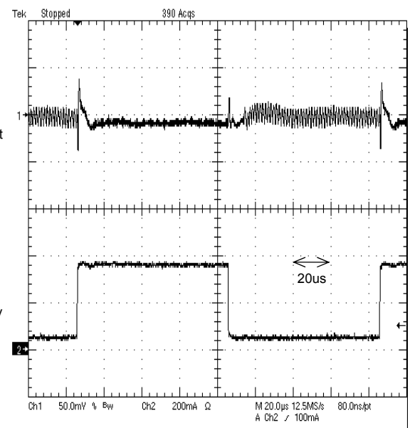
Figure 8. Load transient response 50mA to 350mA t_r=t_f=100\text{ns} , MODE : Low
