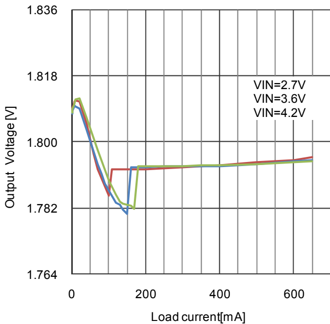
Figure 35. Load regulation PWM/PFM Auto mode
