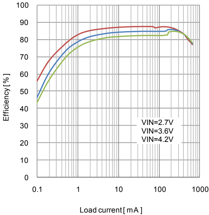
Figure 49. Efficiency vs Load current PWM/PFM Auto mode
