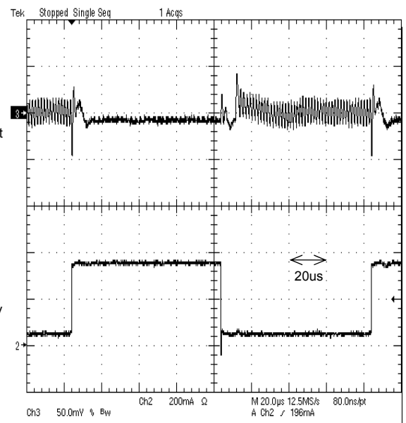
Figure 24. Load transient response 50mA to 350mA t_r=t_f=100\text{ns} , MODE : Low
