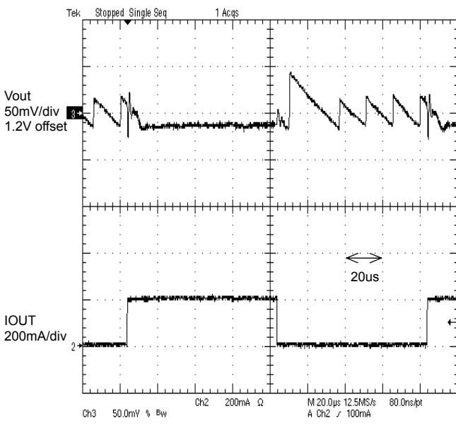
Figure 23. Load transient response 5mA to 200mA t_r=t_f=100\text{ns} , MODE : Low
