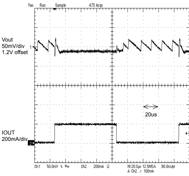
Figure 7. Load transient response 5mA to 200mA t_r=t_f=100\text{ns} , MODE : Low
