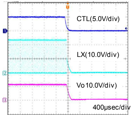
Fig.25 Stop (Rload=2.5Ω)
