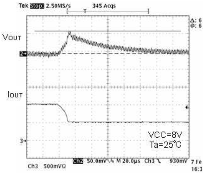
Fig.18 Transient response I_o=1\text{A} \rightarrow 0.5\text{A} (10µs)
