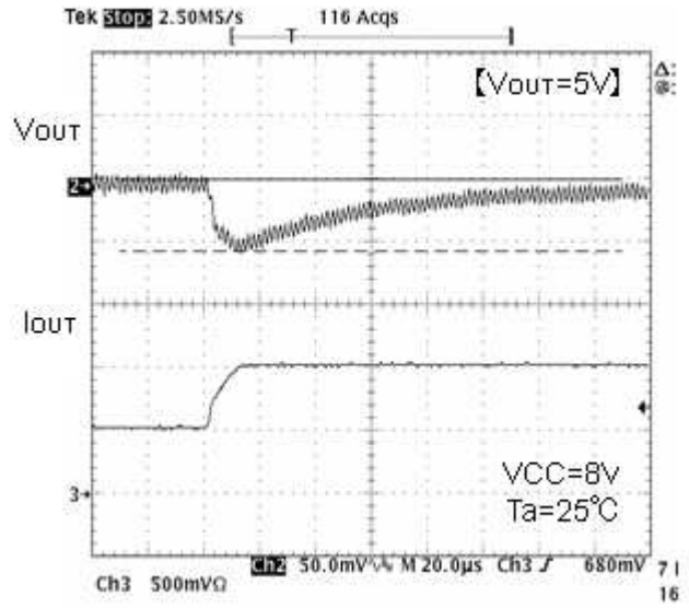
Fig.17 Transient response I_o=0.5\text{A} \rightarrow 1\text{A} (10µs)
