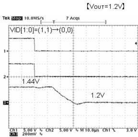
Fig.20 Change Response
