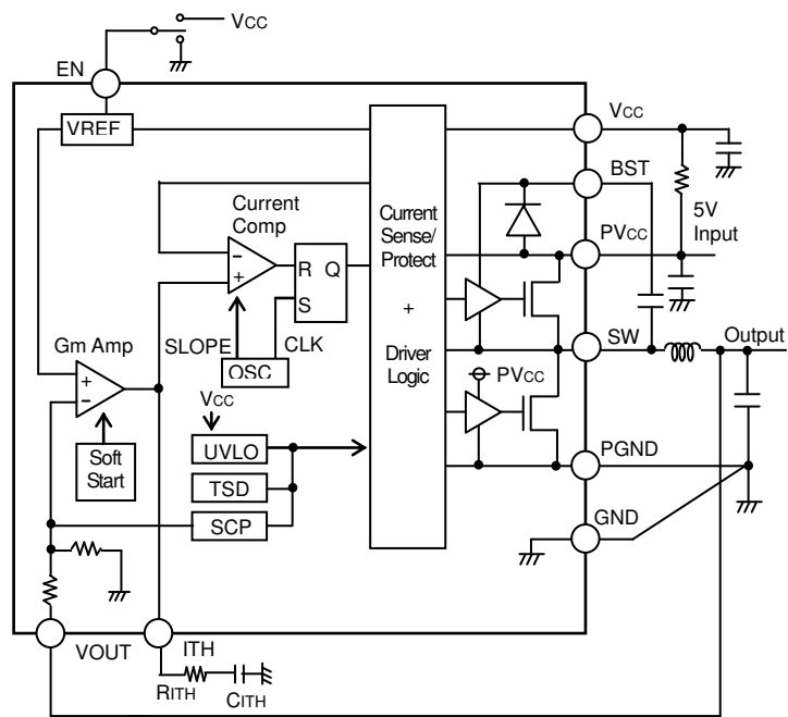
Fig.3 Block Diagram
