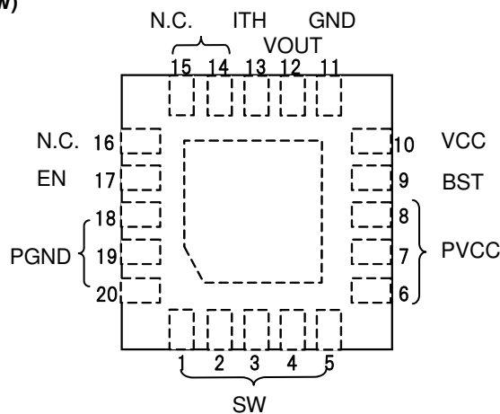
Fig.2 Pin configuration
