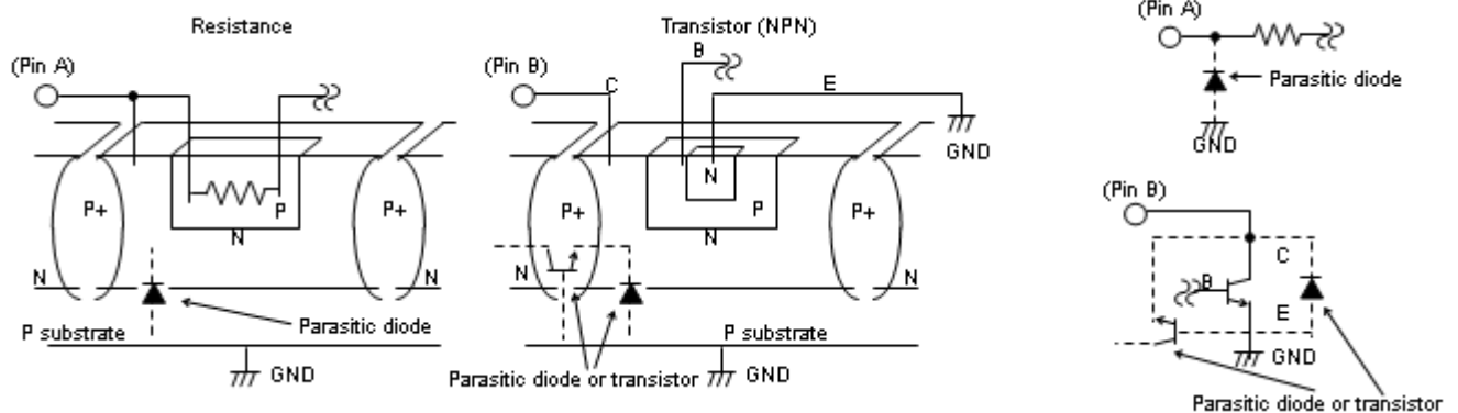
Fig.60 Simplified structure of monorisc IC
