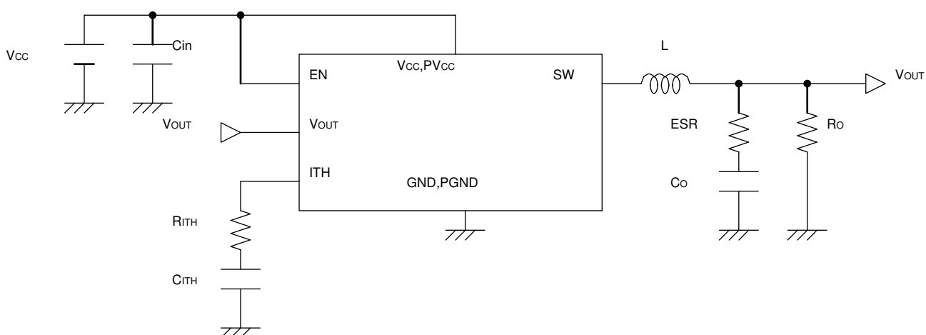
Fig.1 Typical Application Circuit
